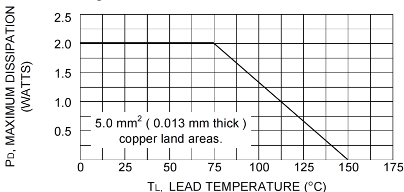
Fig. 1 POWER TEMPERATURE DERATING CURVE
